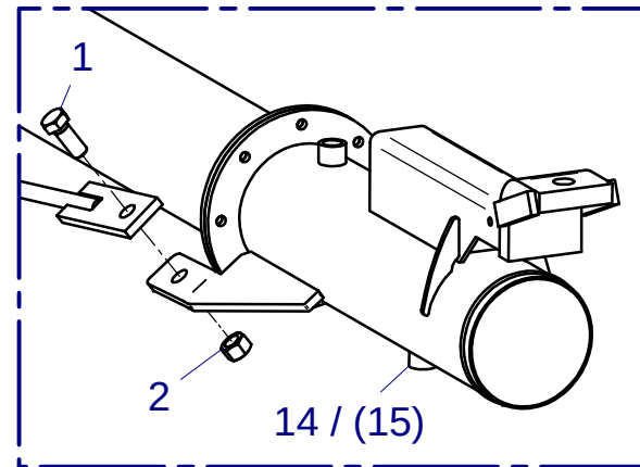
Detail F
