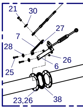
Detail E
