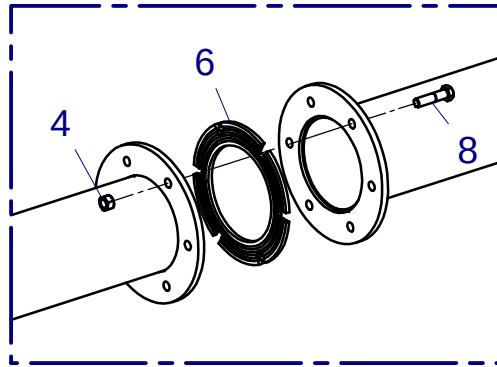
Detail B
